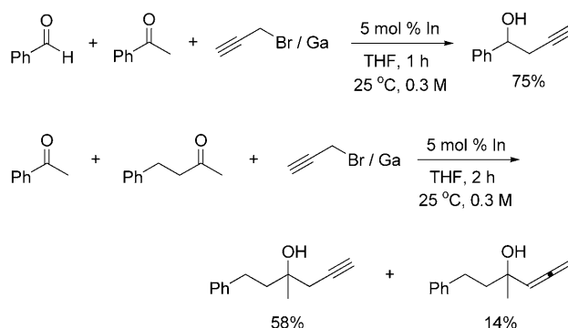
Scheme 2. Competition reaction of benzaldehyde and acetophenone and acetophenone and 4-phenyl-2-butanone under the present conditions.
